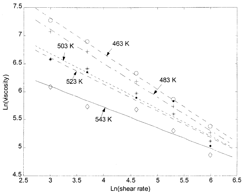
Figure 3 Plots of \ln \eta against \ln \dot{\gamma} for PP at the following temperatures: (○) 463, (+) 483, (*) 503, (●) 523, and (◇) 543 K.
